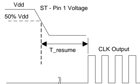
Figure 6. Resume Timing [5, 6]
